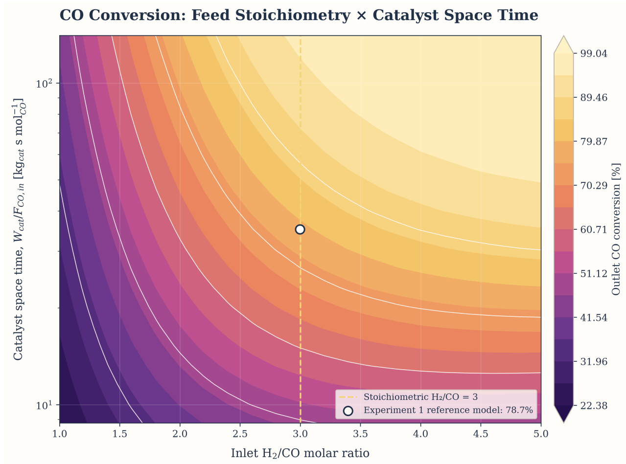
Figure 5. Full M4 predicted outlet CO conversion at 1 bar as inlet H 2 /CO ratio and catalyst space time vary.
